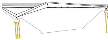
▲ East elevation drawing. ◀ General view of the structure.
